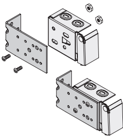
End Bracket with 2" Extension Bracket
